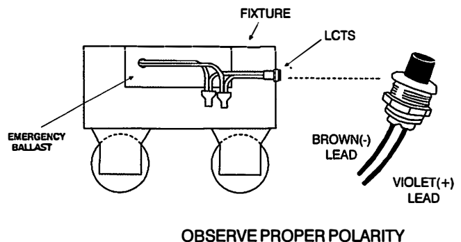
Illustration 2 Strip Fixture
